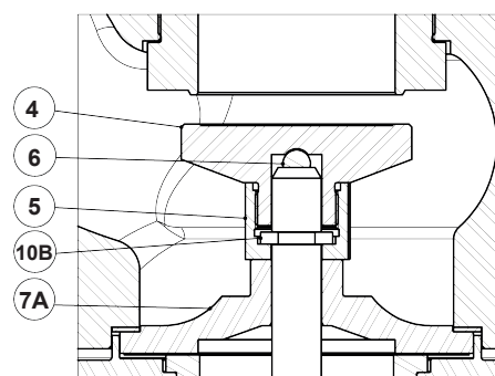
Detail A (DN 80 - DN 100)
